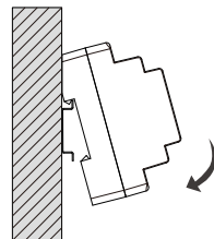
Mounting method 2: DIN nail mounting. Slot the DCU on the DIN nail.
